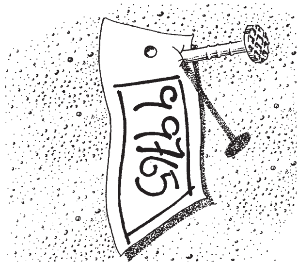
intensive stratification
