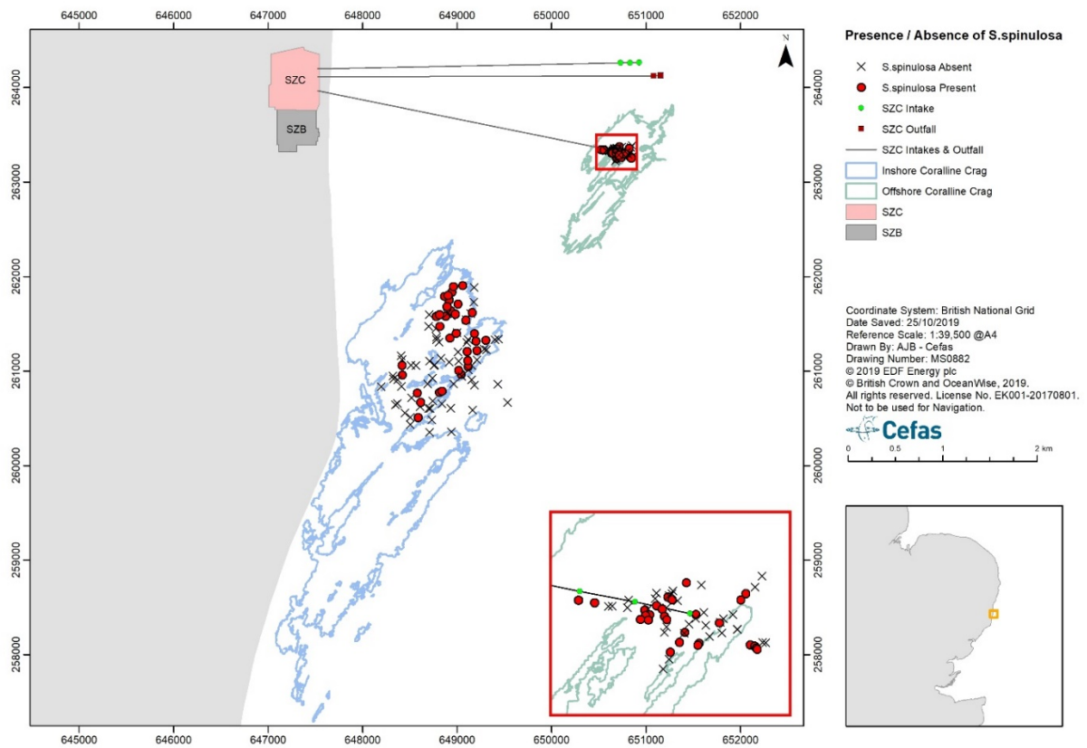
Figure 2.1: Extent of the inshore and offshore Coralline Crag and the location of ground-truthing sampling stations. Sabellaria spinulosa aggregations were identified from the acoustic image footage at both sites (red points).
