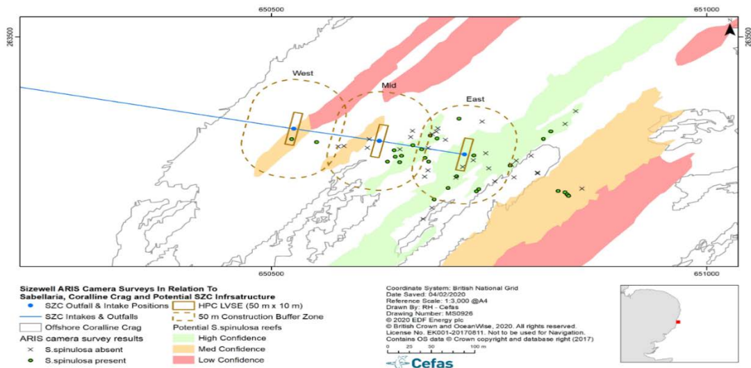
Figure 3.1: Locations of Unit 1 cooling water intake head position options (two to be installed) at the offshore Coralline Crag. Headworks and a 50m construction buffer zone are shown relative to the predicted extent of potential S. spinulosa reef of at least ‘medium’ quality (BEEMS Technical Report TR512). Confidence is based on a combination of the acoustic signal from side-scan sonar and the amount of ground-truthing support. Reef identified to any confidence level was assumed to be reef for the purposes of the assessment.
